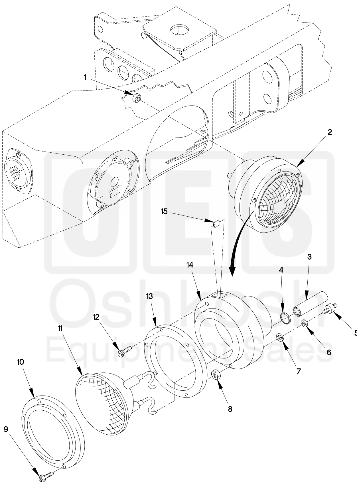
FIGURE 66. HEADLAMP ASSEMBLY
